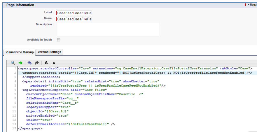
Figure 2 CaseFeedCaseFilePage
